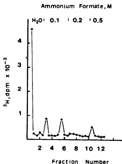
Fig.3. Analysis by Dowex AG1 \times 8 chromatography of peak III from fig.2 after treatment with alkaline phosphatase. Peak III from fig.2 was lyophilized, treated with alkaline phosphatase (25 mM Tris-HCl, pH 8.3, containing 5 U/ml, for 2 h at 37°C), applied to a Dowex AG1 \times 8 column (2 ml bed volume), and after washing with water, eluted with various concentrations of ammonium formate. After elution, the amount of radioactivity in each fraction (2 ml) was determined by counting an aliquot.
