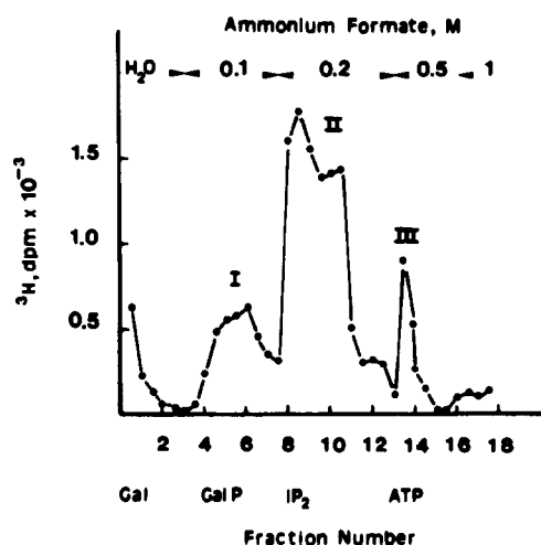
Fig.2. Analysis by Dowex AG1 \times 8 chromatography of the aqueous products after treatment of [ ^3\text{H} ]galactose-labeled glycosyl-PI with PI-PIC. A sample of [ ^3\text{H} ]galactose-labeled glycosyl-PI was treated with PI-PIC (see text). After hydrolysis, the aqueous fraction was applied to a Dowex AG1 \times 8 column (2 ml bed volume) and, after washing the column with water, eluted with various concentrations of ammonium formate. After elution, the amount of radioactivity in each fraction (2 ml) was determined by counting an aliquot. Gal, galactose; GalP, galactose 1-phosphate; IP 2 , inositol 1,4-bisphosphate; ATP, adenosine triphosphate. Migration positions of the known substances were determined with markers.
